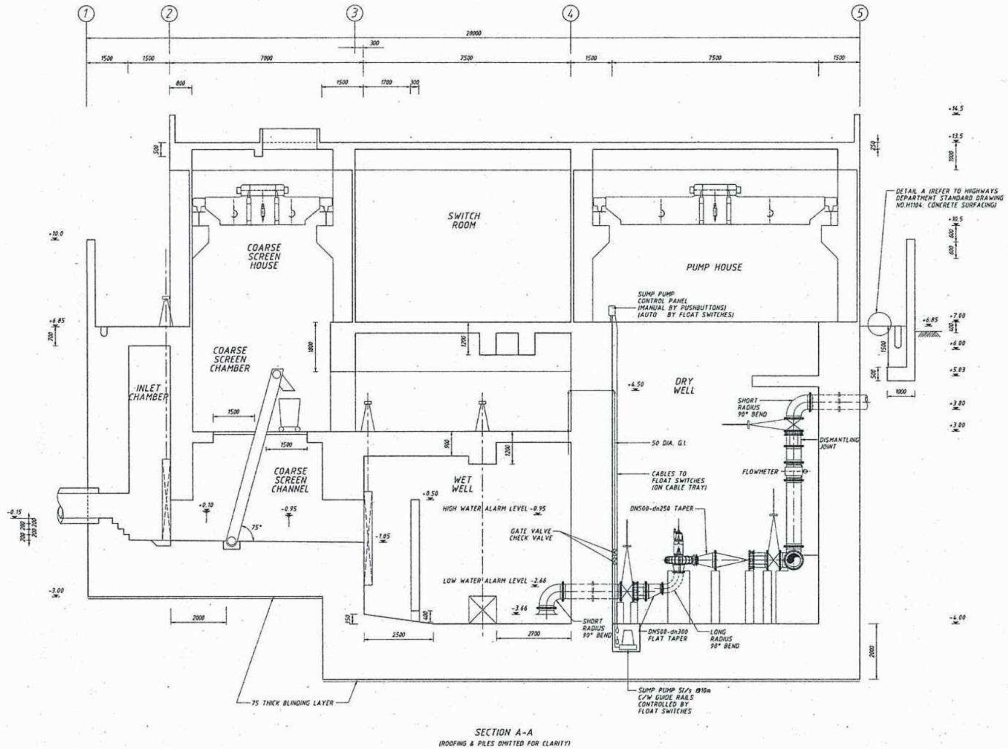
Figure 5: Sewage Pumping Station and Equalization Tanks - Sections
